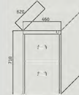
Model No: SS020 W460 x D620 x H710
