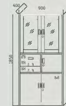
Model No: SS014 W900 x D400 x H1850
