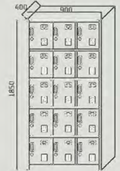
Model No: SS033 W900 x D400 x H1850
