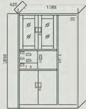
Model No: SS0010 W1180 x D420 x H1850
