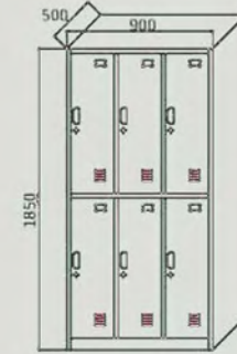
Model No: SS027 W900 x D500 x H1850
